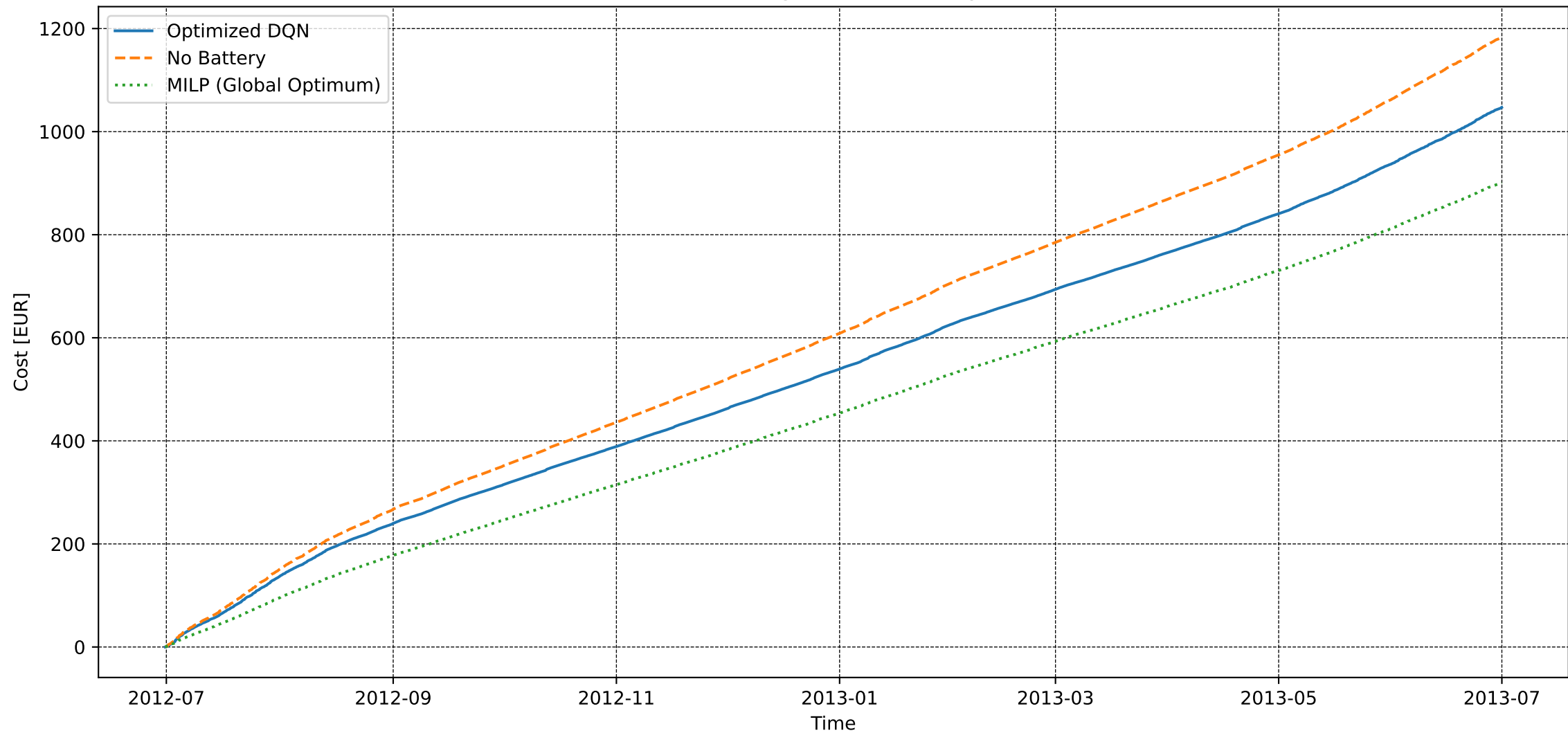
User 179 - Extended Convergence - Electricity Cost [DQN vs MILP]
